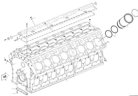
CRANKCASE UPC.06A01 0791
