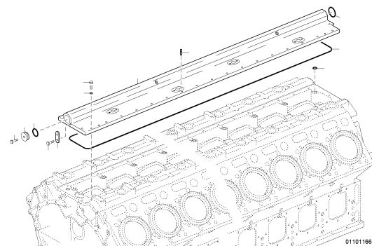
TOP VALLEY COVER SINGLE PASSAGE INDUSTRI UPC.06A01D0015
